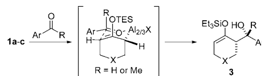
Figure 1. Proposed transition state for the diastereoselective additions of 1a–c to aldehydes and methyl ketones.
