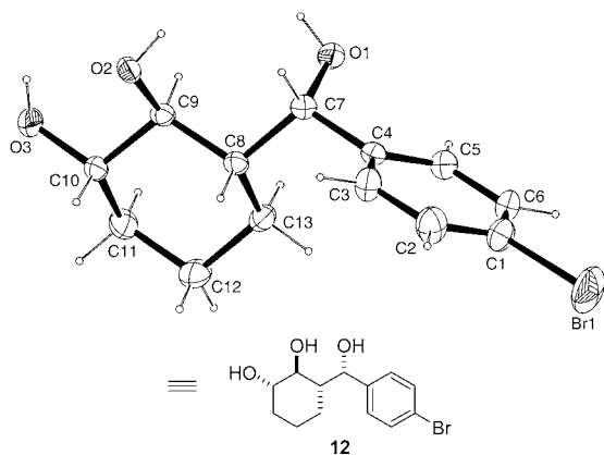
Figure 2. X-ray crystal structure of triol 12.
